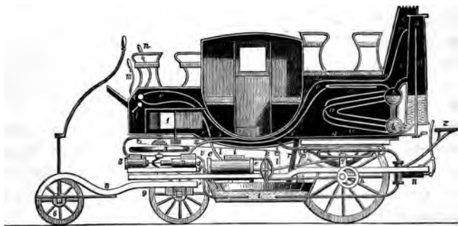
FIG. 48.—Gurney's Steam-Carriage.
